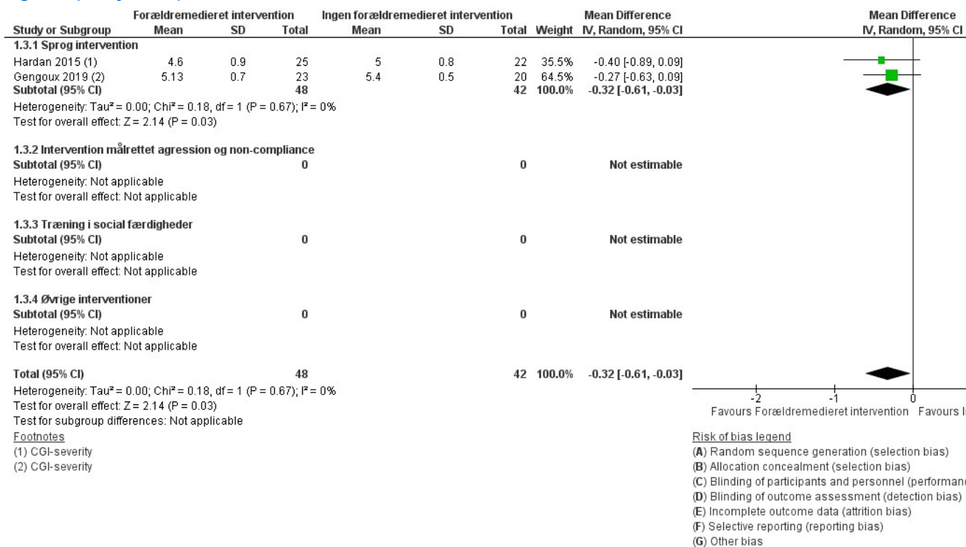
Figure 3 (Analysis 1.3)
