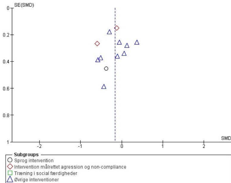
Figure 10 (Analysis 1.7)
