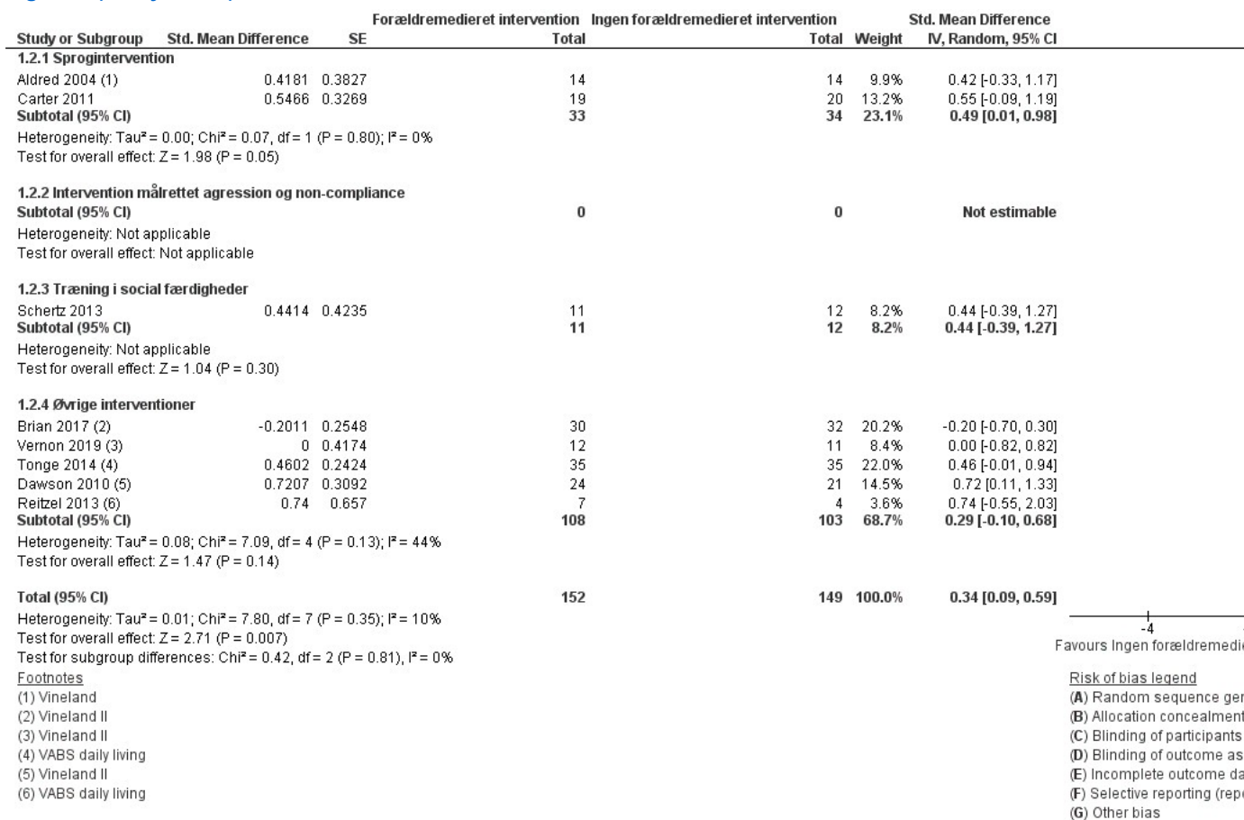
Figure 2 (Analysis 1.2)
