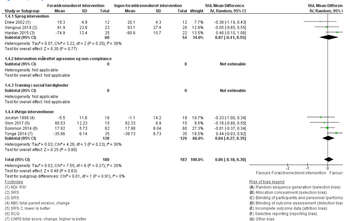
Figure 4 (Analysis 1.4)
